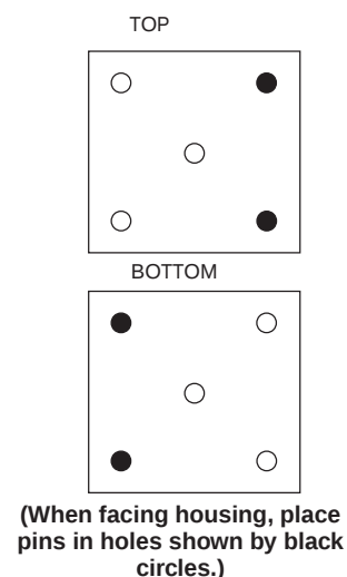
AS-B821-108 Mechanical Keying for Housings
