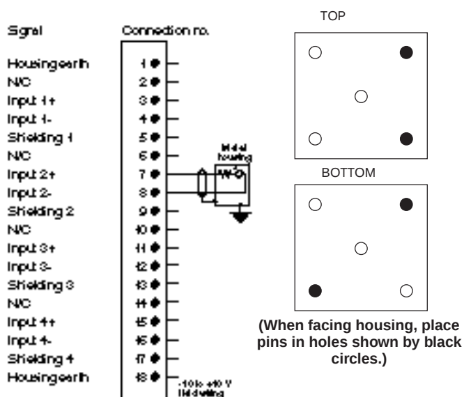
AS-B873-011 Terminal Numbering and Wire Connections
