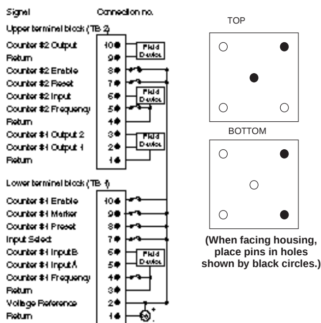
AS-B883-001 Terminal Numbering and Wire Connections
