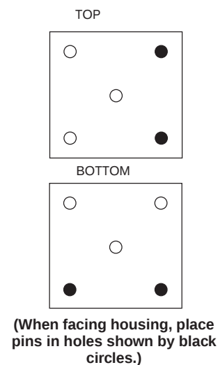
AS-B827-032 Mechanical Keying for Housings
