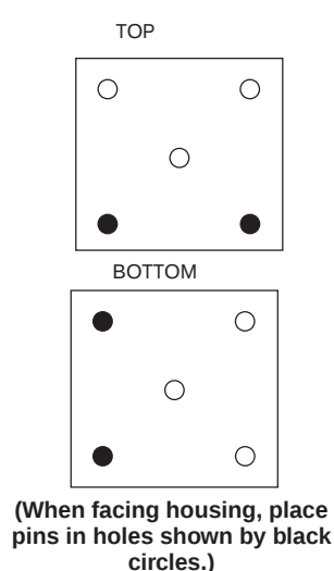
AS-B820-008 Mechanical Keying for Housings
