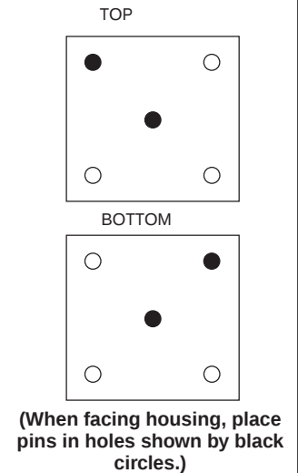
AS-B881-108 Mechanical Keying for Housings
