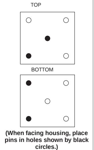
AS-B837-016 Mechanical Keying for Housings
