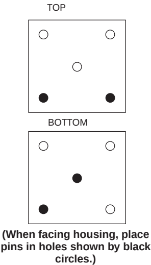
AS-B882-116 Mechanical Keying for Housings
