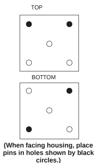
AS-B855-016 Mechanical Keying for Housings
