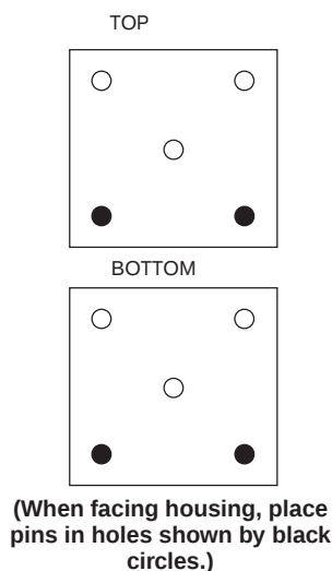
AS-B826-032 Mechanical Keying for Housings
