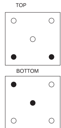
AS-B872-100 Mechanical Keying for Housings
