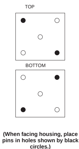
AS-B832-016 Mechanical Keying for Housings
