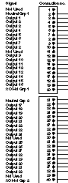
AS-B806-032 Terminal Numbering and Wire Connections
