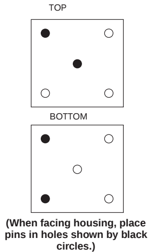
AS-B836-016 Mechanical Keying for Housings
