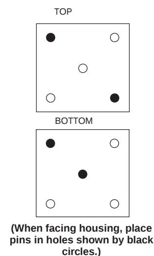
AS-B863-032 Mechanical Keying for Housings
