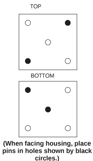
AS-B875-200 Mechanical Keying for Housings
