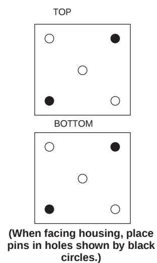
AS-B833-016 Mechanical Keying for Housings
