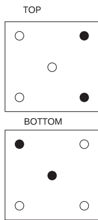
AS-B872-200 Mechanical Keying for Housings
