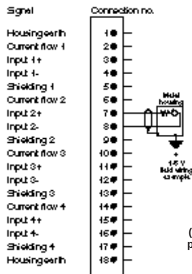
AS-B873-001 Terminal Numbering and Wire Connections
