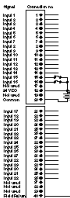
AS-B863-032 Terminal Numbering and Wire Connections
